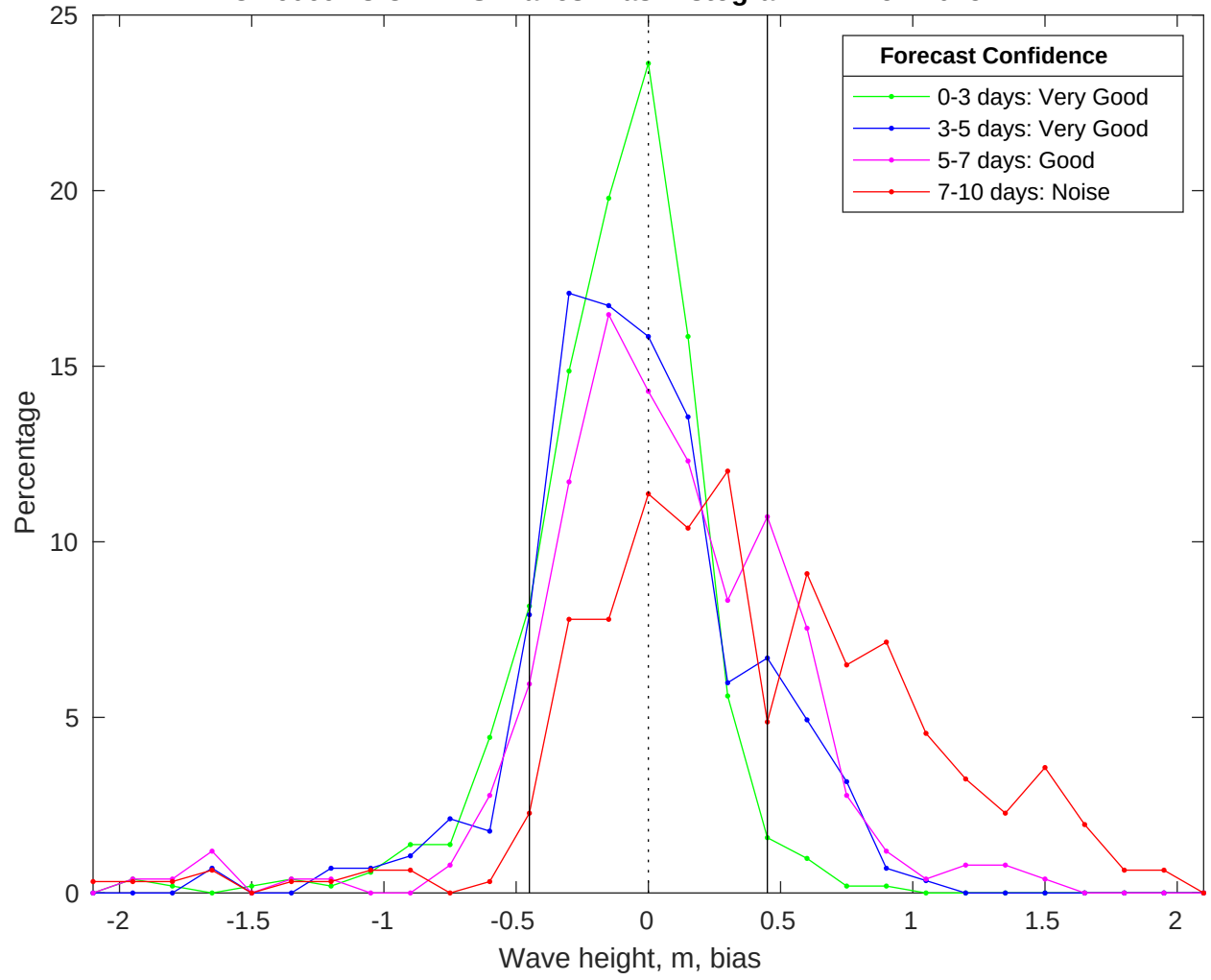
NDBC 46069 vs CMEMS Waves Bias Histogram: 22-Nov-2025
