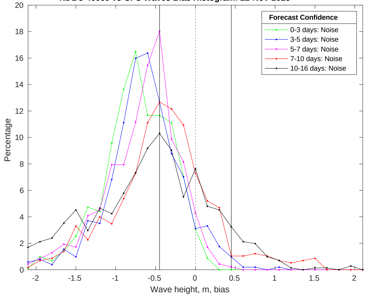
NDBC 46069 vs GFS Waves Bias Histogram: 22-Nov-2025
