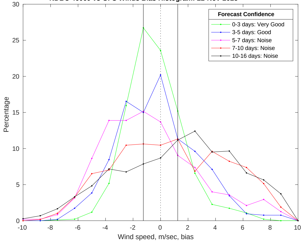
NDBC 46069 vs GFS Winds Bias Histogram: 22-Nov-2025
