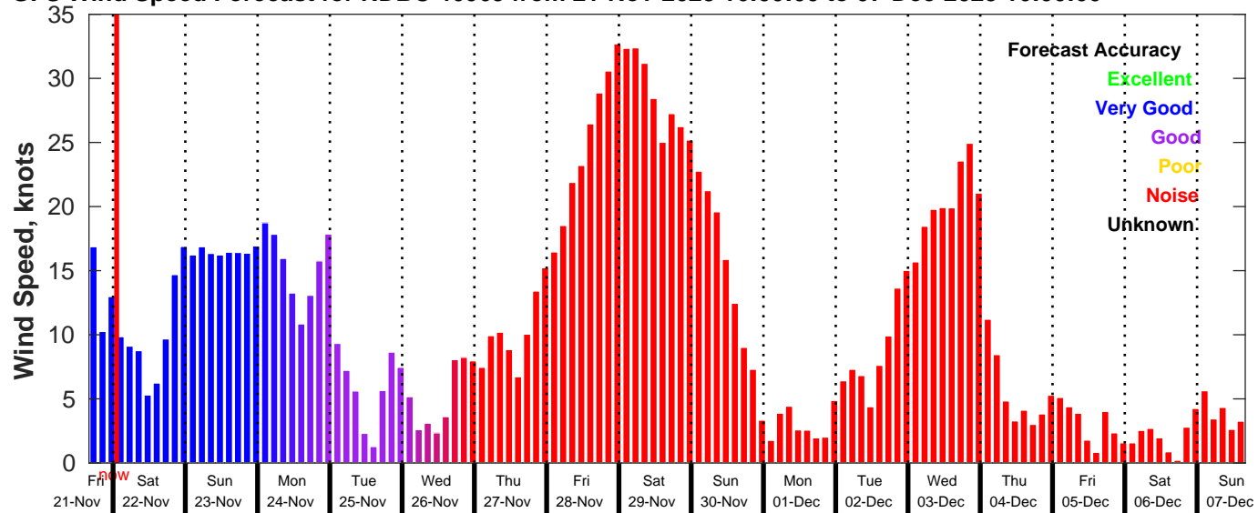
GFS Wind Speed Forecast for NDBC 46069 from 21-Nov-2025 16:00:00 to 07-Dec-2025 16:00:00
