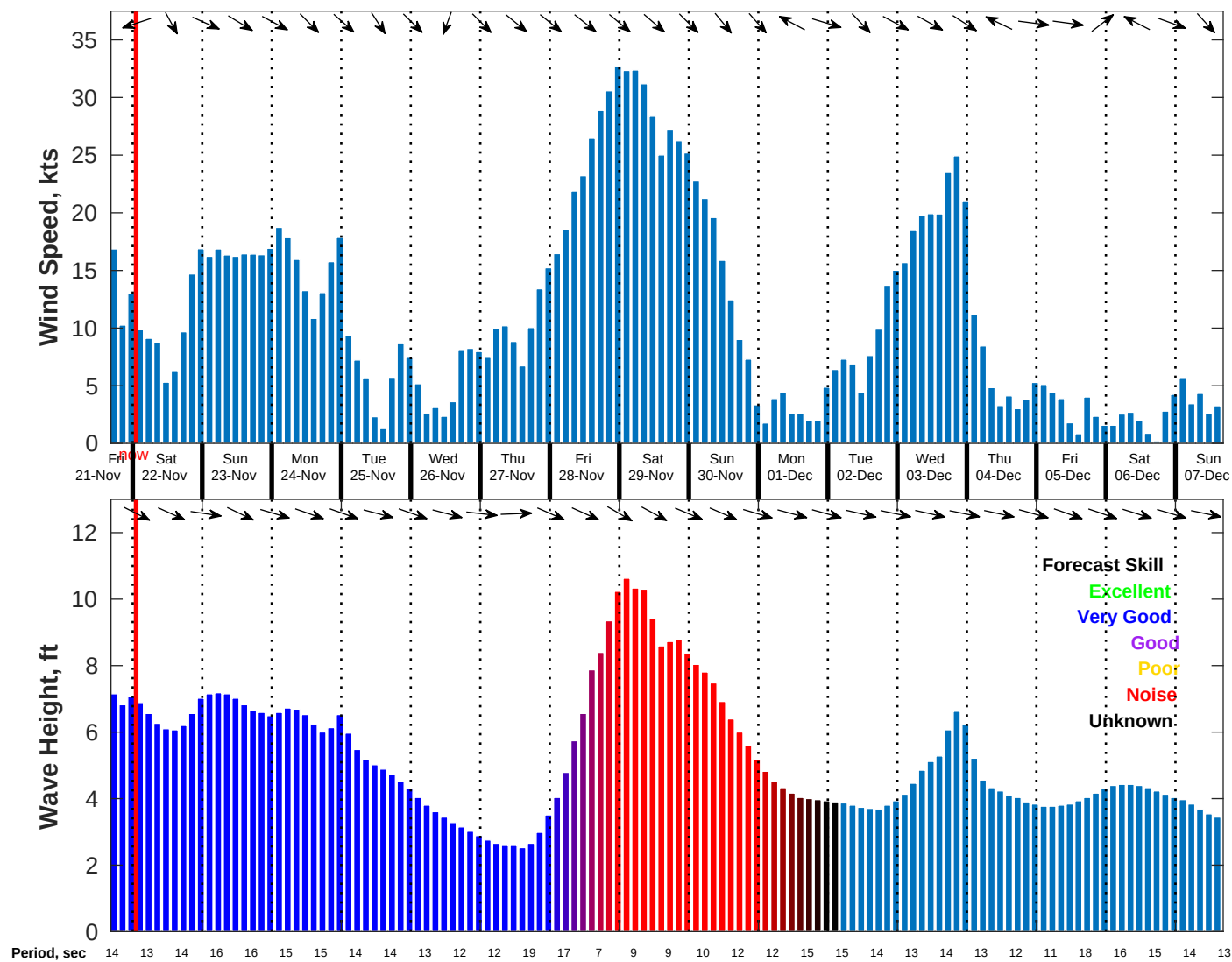
Wind & Wave Forecast for NDBC 46069 from 21-Nov-2025 16:00:00 to 07-Dec-2025 16:00:00
