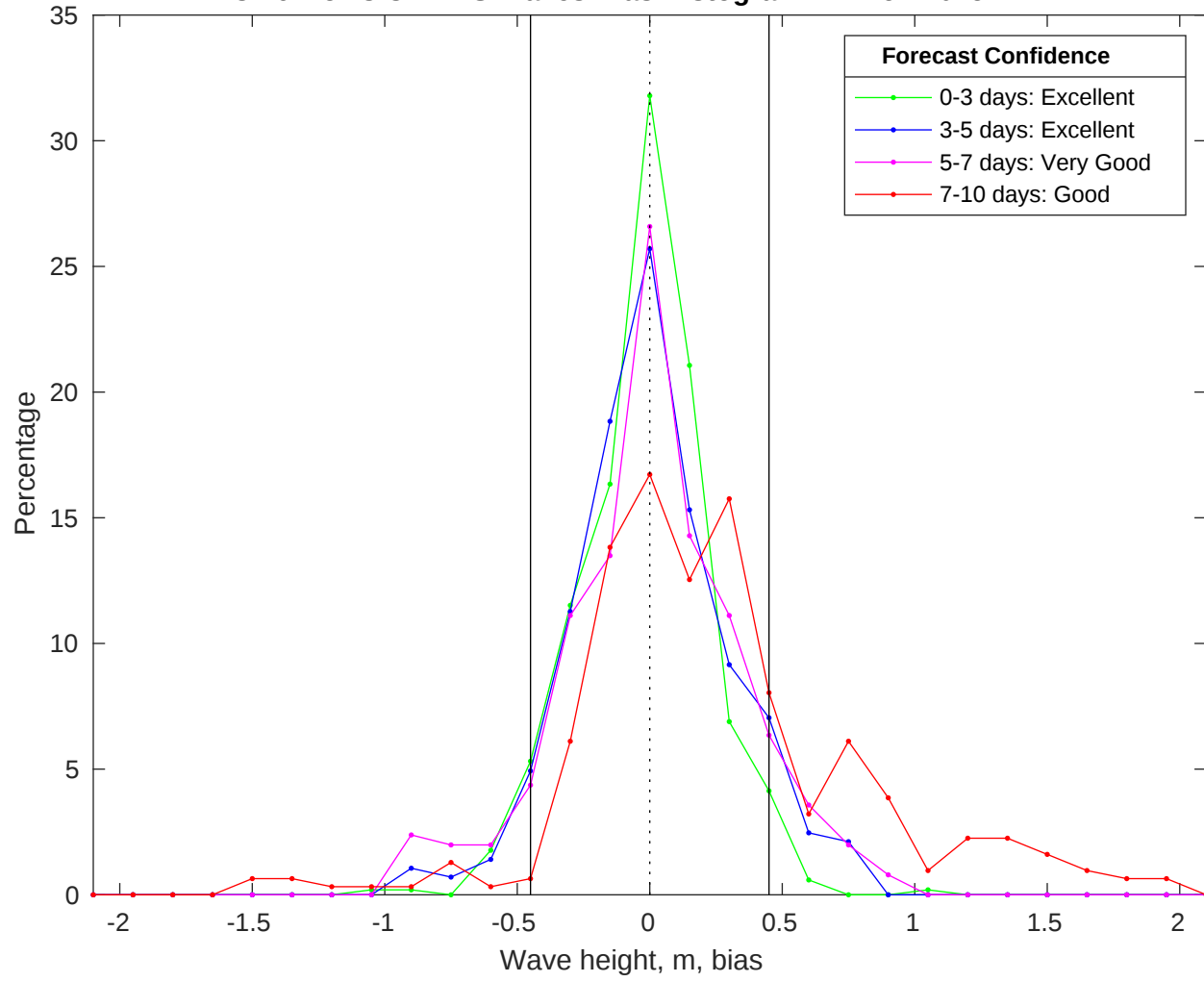
NDBC 46215 vs CMEMS Waves Bias Histogram: 22-Nov-2025
