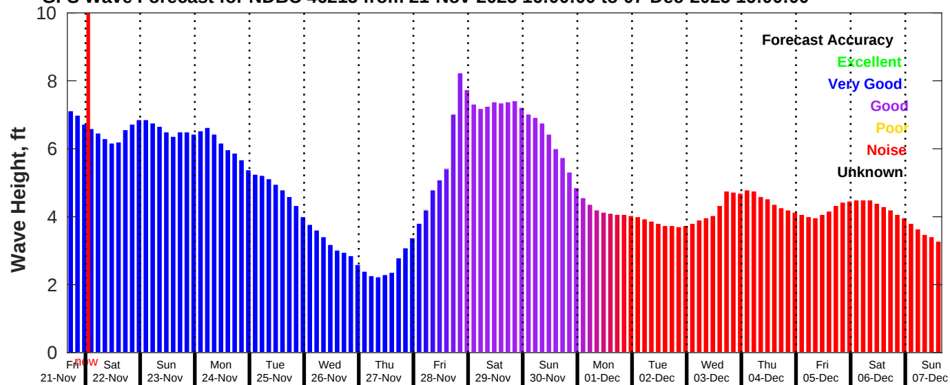
GFS Wave Forecast for NDBC 46215 from 21-Nov-2025 16:00:00 to 07-Dec-2025 16:00:00
