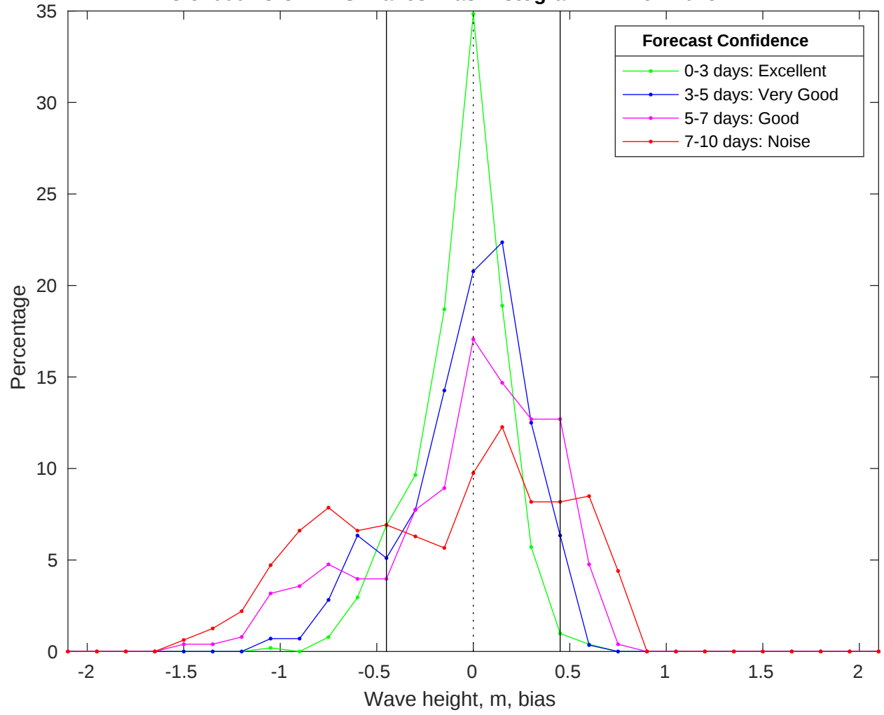
NDBC 51000 vs CMEMS Waves Bias Histogram: 22-Nov-2025
