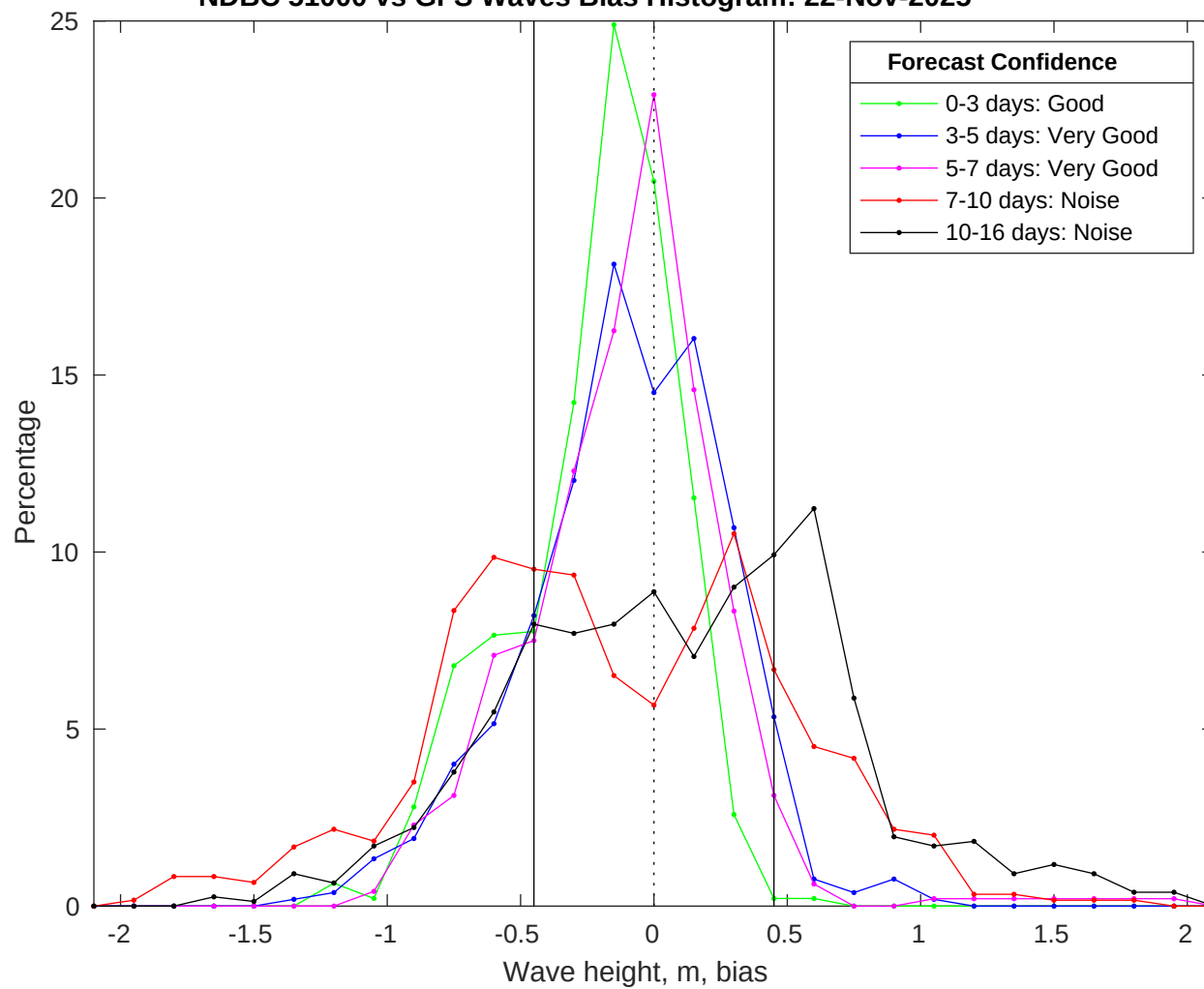
NDBC 51000 vs GFS Waves Bias Histogram: 22-Nov-2025
