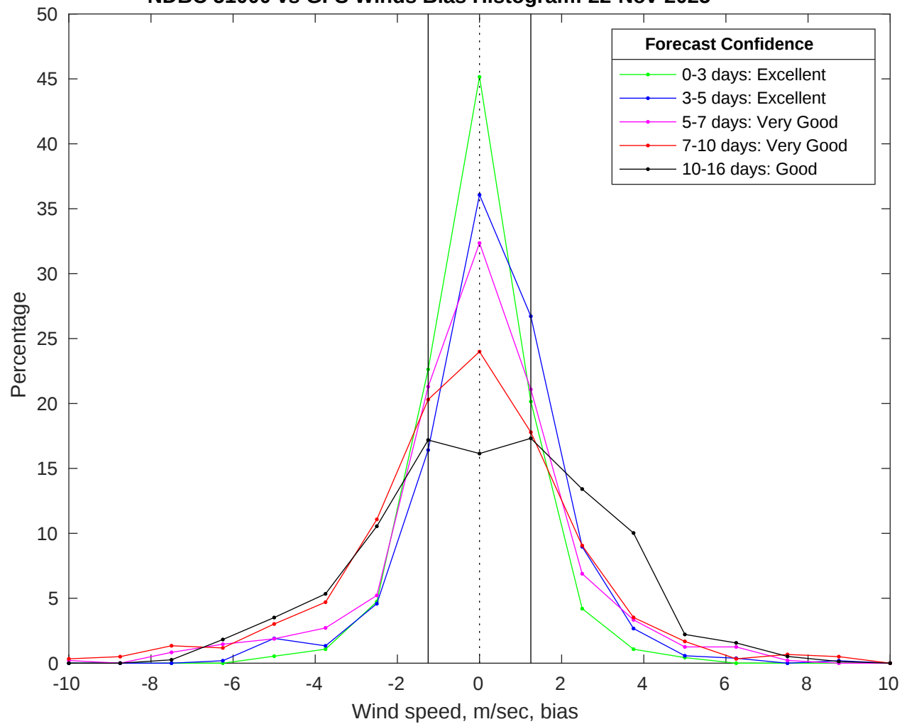
NDBC 51000 vs GFS Winds Bias Histogram: 22-Nov-2025
