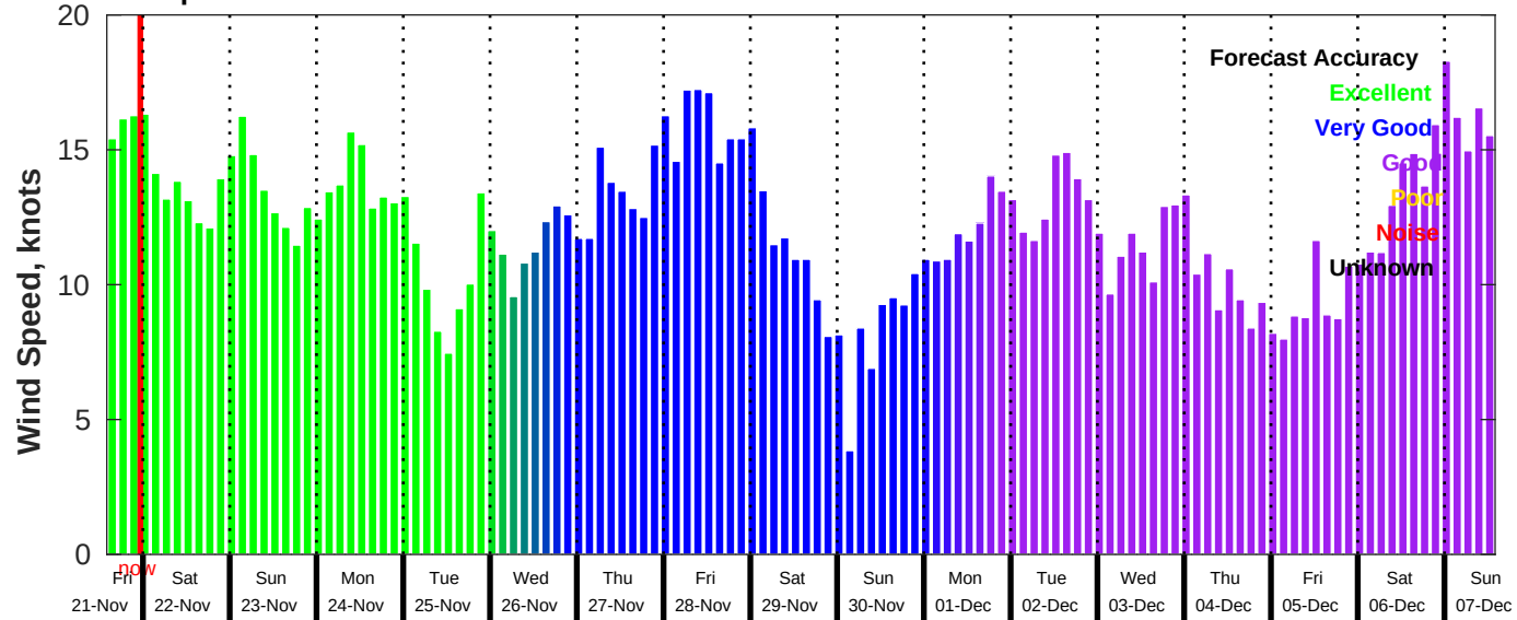
GFS Wind Speed Forecast for NDBC 51000 from 21-Nov-2025 14:00:00 to 07-Dec-2025 14:00:00
