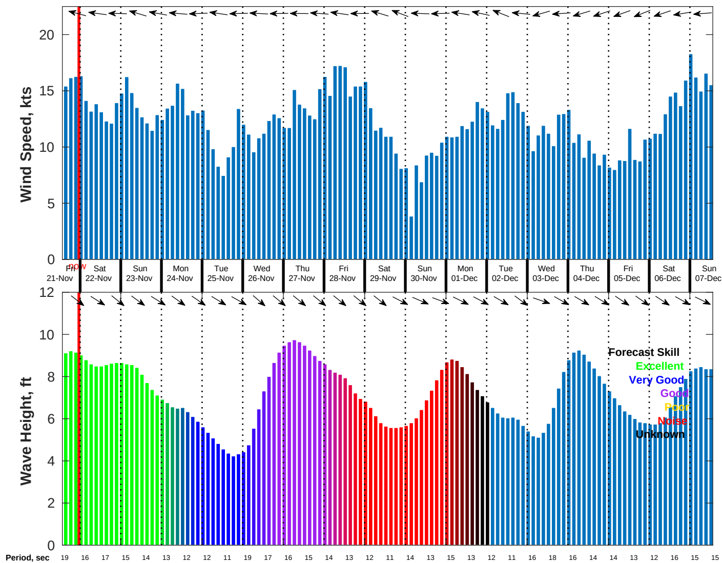
Wind & Wave Forecast for NDBC 51000 from 21-Nov-2025 14:00:00 to 07-Dec-2025 14:00:00
