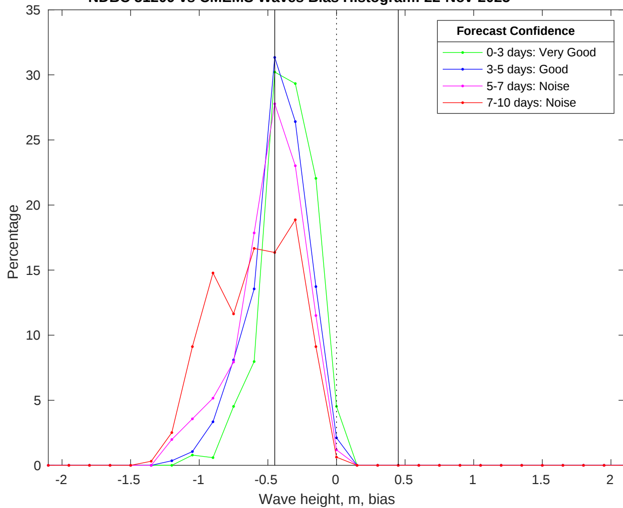
NDBC 51209 vs CMEMS Waves Bias Histogram: 22-Nov-2025
