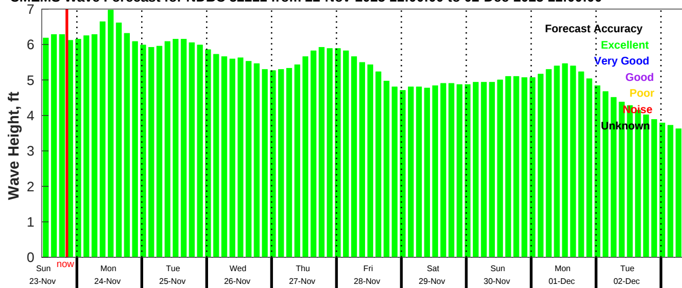
CMEMS Wave Forecast for NDBC 52211 from 22-Nov-2025 11:00:00 to 02-Dec-2025 11:00:00
