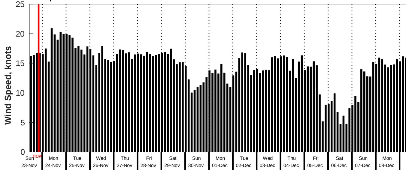
GFS Wind Speed Forecast for NDBC 52211 from 22-Nov-2025 11:00:00 to 08-Dec-2025 11:00:00
