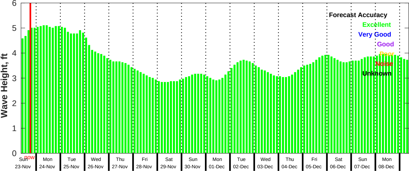
GFS Wave Forecast for NDBC 52212 from 22-Nov-2025 09:00:00 to 08-Dec-2025 09:00:00
