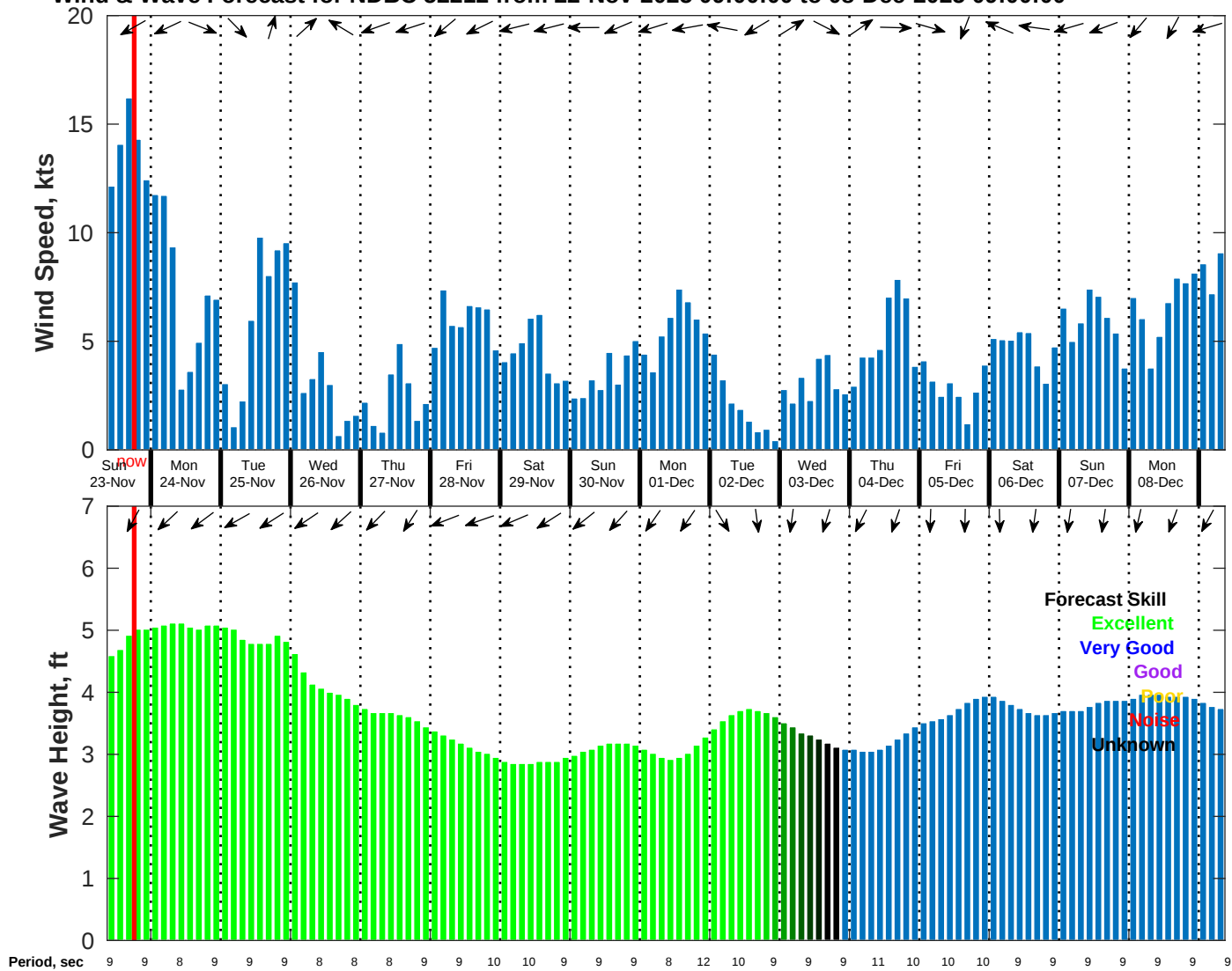
Wind & Wave Forecast for NDBC 52212 from 22-Nov-2025 09:00:00 to 08-Dec-2025 09:00:00
