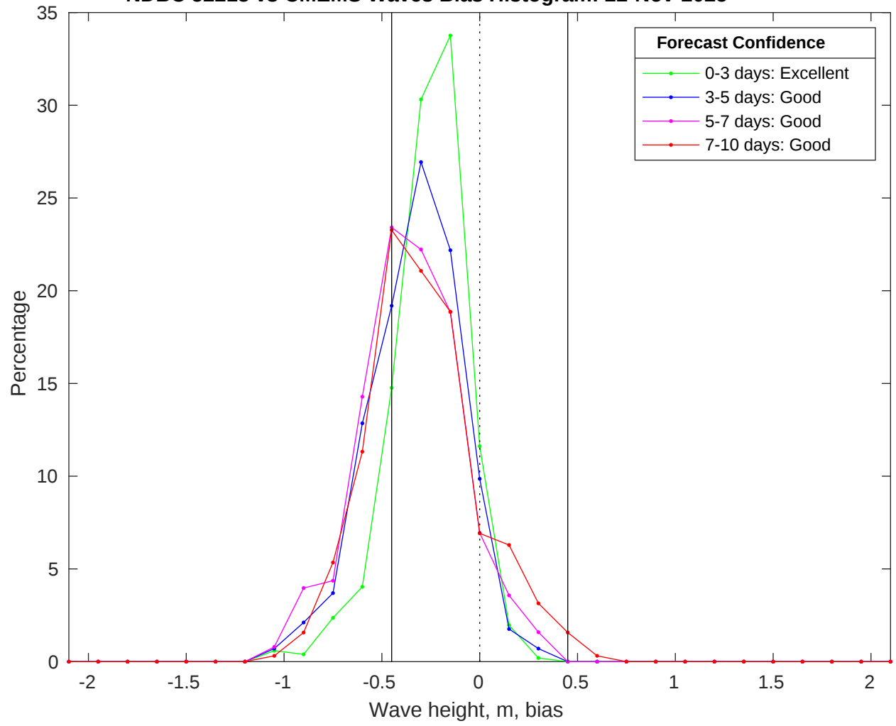
NDBC 52213 vs CMEMS Waves Bias Histogram: 22-Nov-2025
