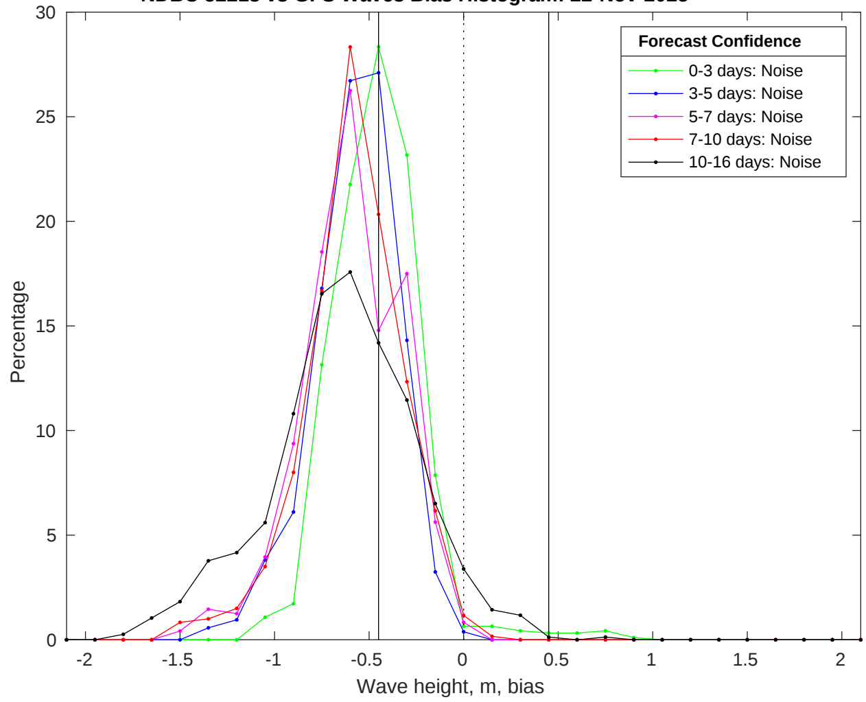
NDBC 52213 vs GFS Waves Bias Histogram: 22-Nov-2025
