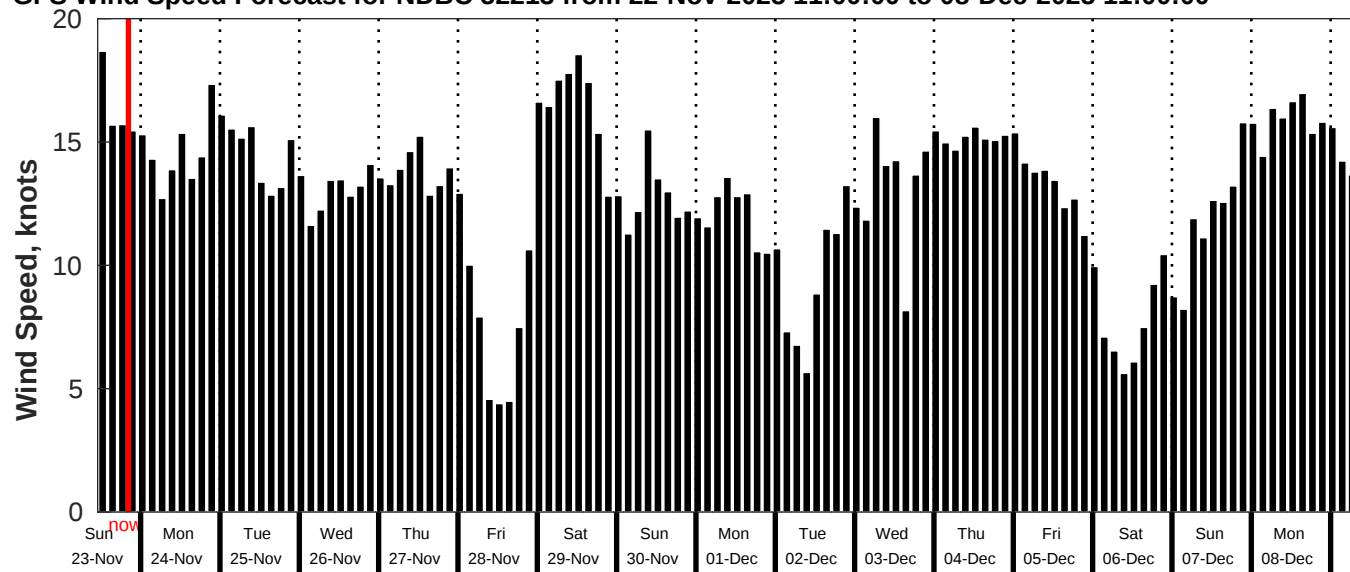
GFS Wind Speed Forecast for NDBC 52213 from 22-Nov-2025 11:00:00 to 08-Dec-2025 11:00:00
