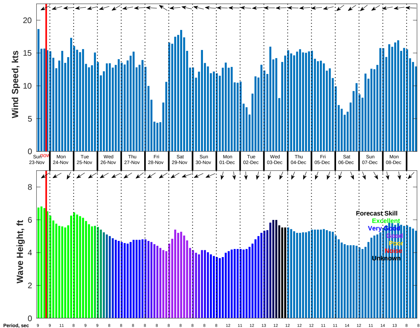
Wind & Wave Forecast for NDBC 52213 from 22-Nov-2025 11:00:00 to 08-Dec-2025 11:00:00
