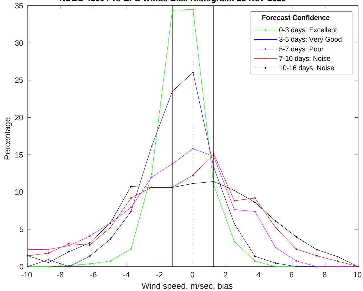
NDBC 41004 vs GFS Winds Bias Histogram: 23-Nov-2025
