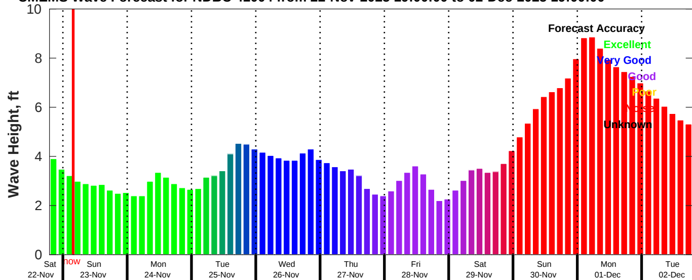
CMEMS Wave Forecast for NDBC 41004 from 22-Nov-2025 19:00:00 to 02-Dec-2025 19:00:00
