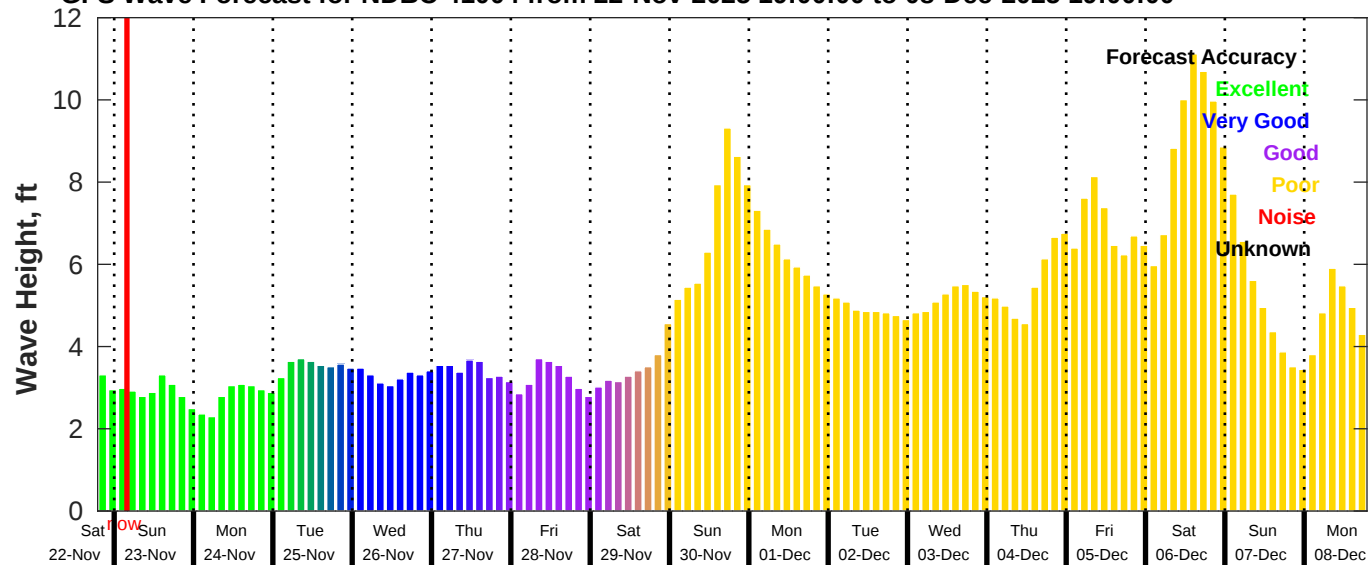
GFS Wave Forecast for NDBC 41004 from 22-Nov-2025 19:00:00 to 08-Dec-2025 19:00:00
