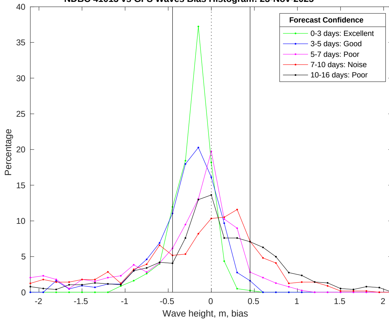
NDBC 41013 vs GFS Waves Bias Histogram: 23-Nov-2025
