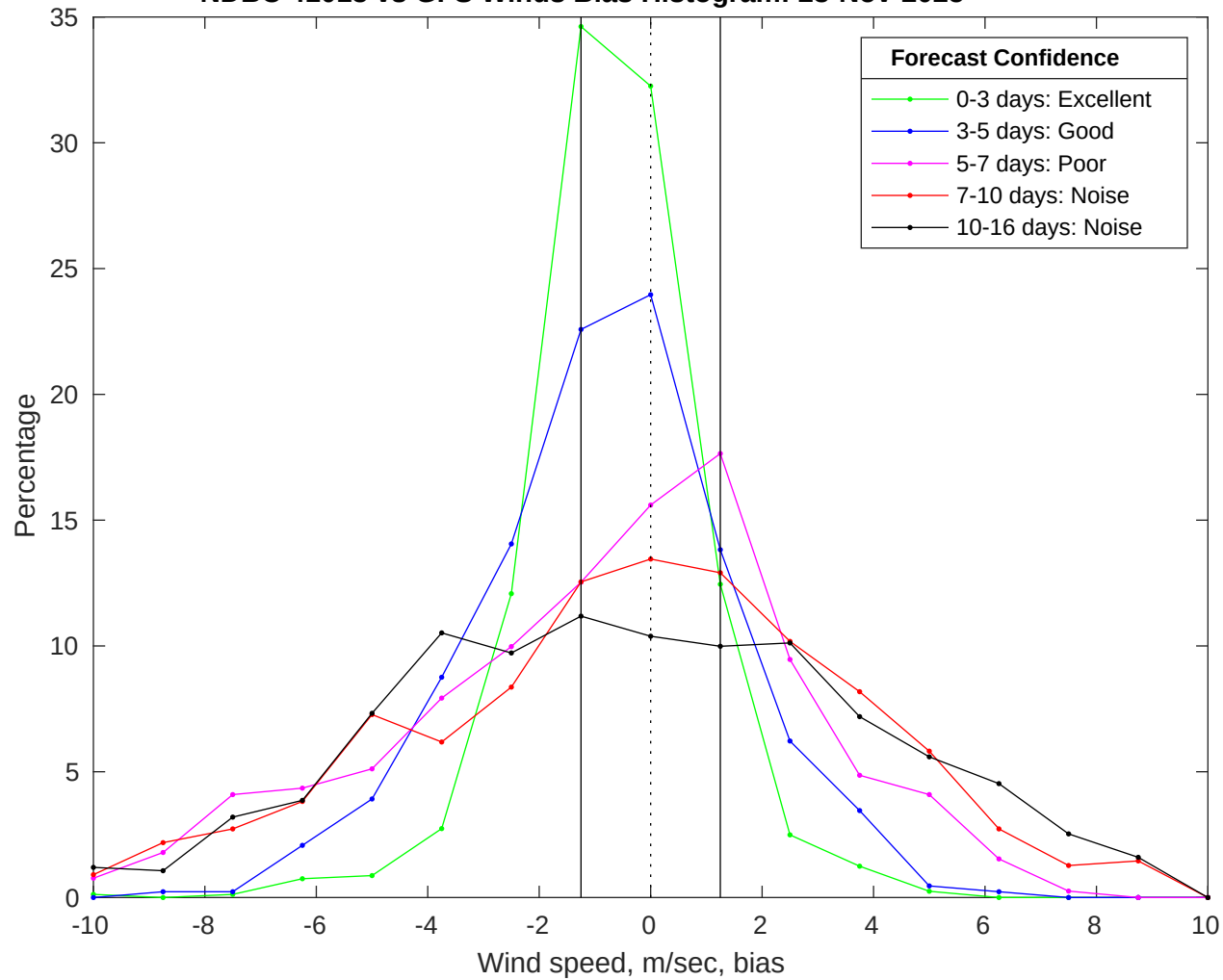
NDBC 41013 vs GFS Winds Bias Histogram: 23-Nov-2025
