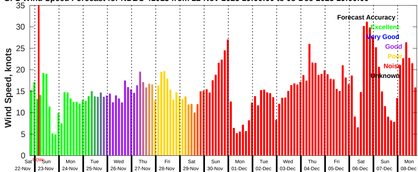
GFS Wind Speed Forecast for NDBC 41013 from 22-Nov-2025 19:00:00 to 08-Dec-2025 19:00:00
