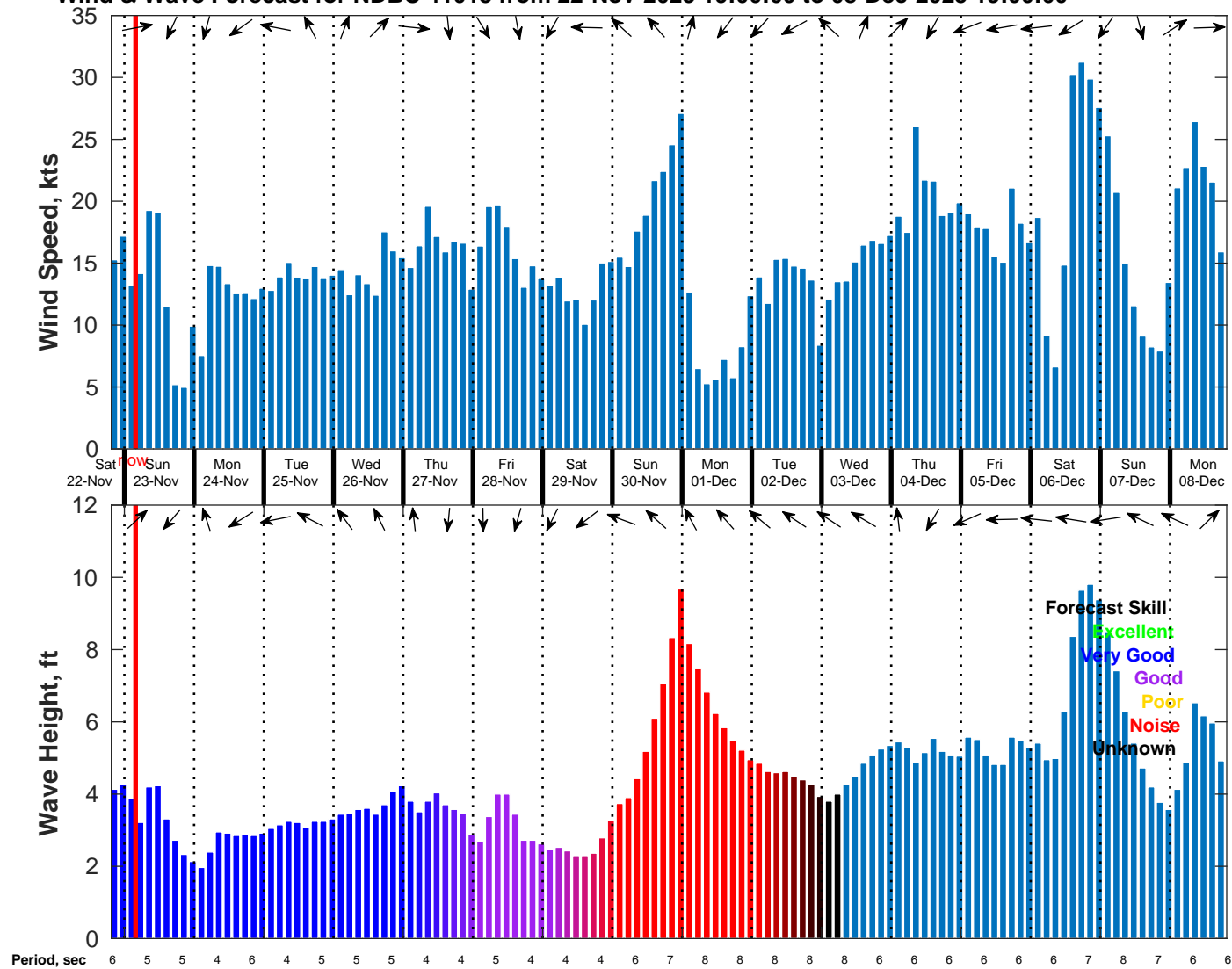
Wind & Wave Forecast for NDBC 41013 from 22-Nov-2025 19:00:00 to 08-Dec-2025 19:00:00
