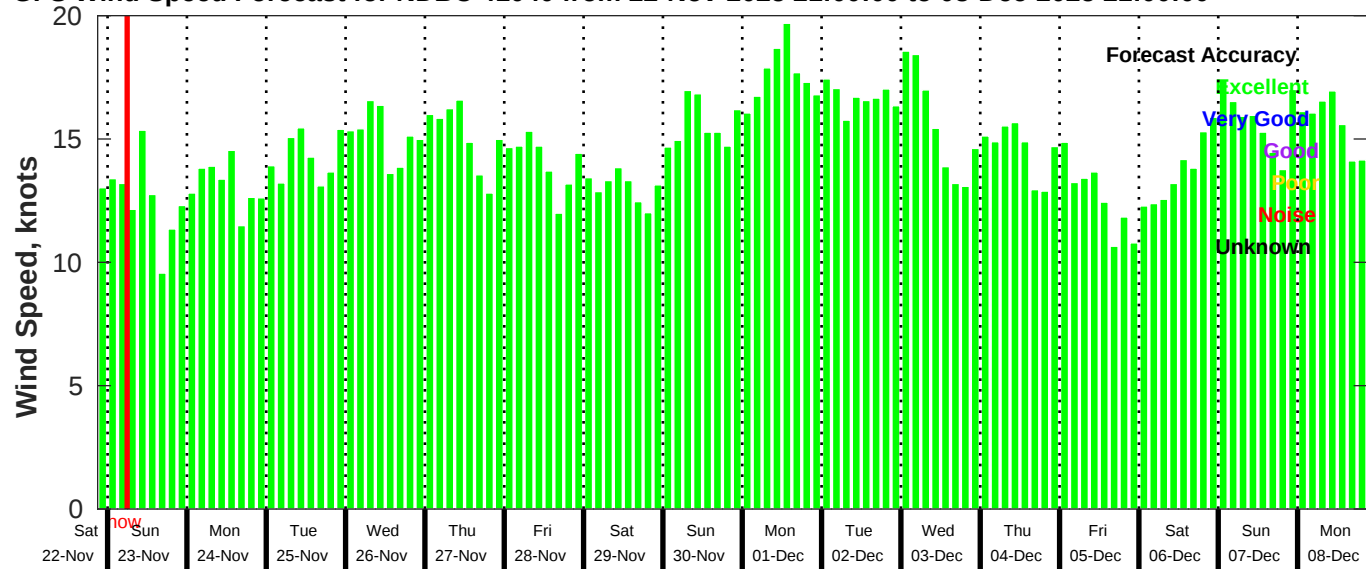
GFS Wind Speed Forecast for NDBC 41040 from 22-Nov-2025 21:00:00 to 08-Dec-2025 21:00:00
