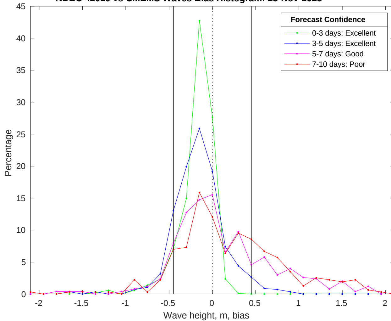
NDBC 42019 vs CMEMS Waves Bias Histogram: 23-Nov-2025
