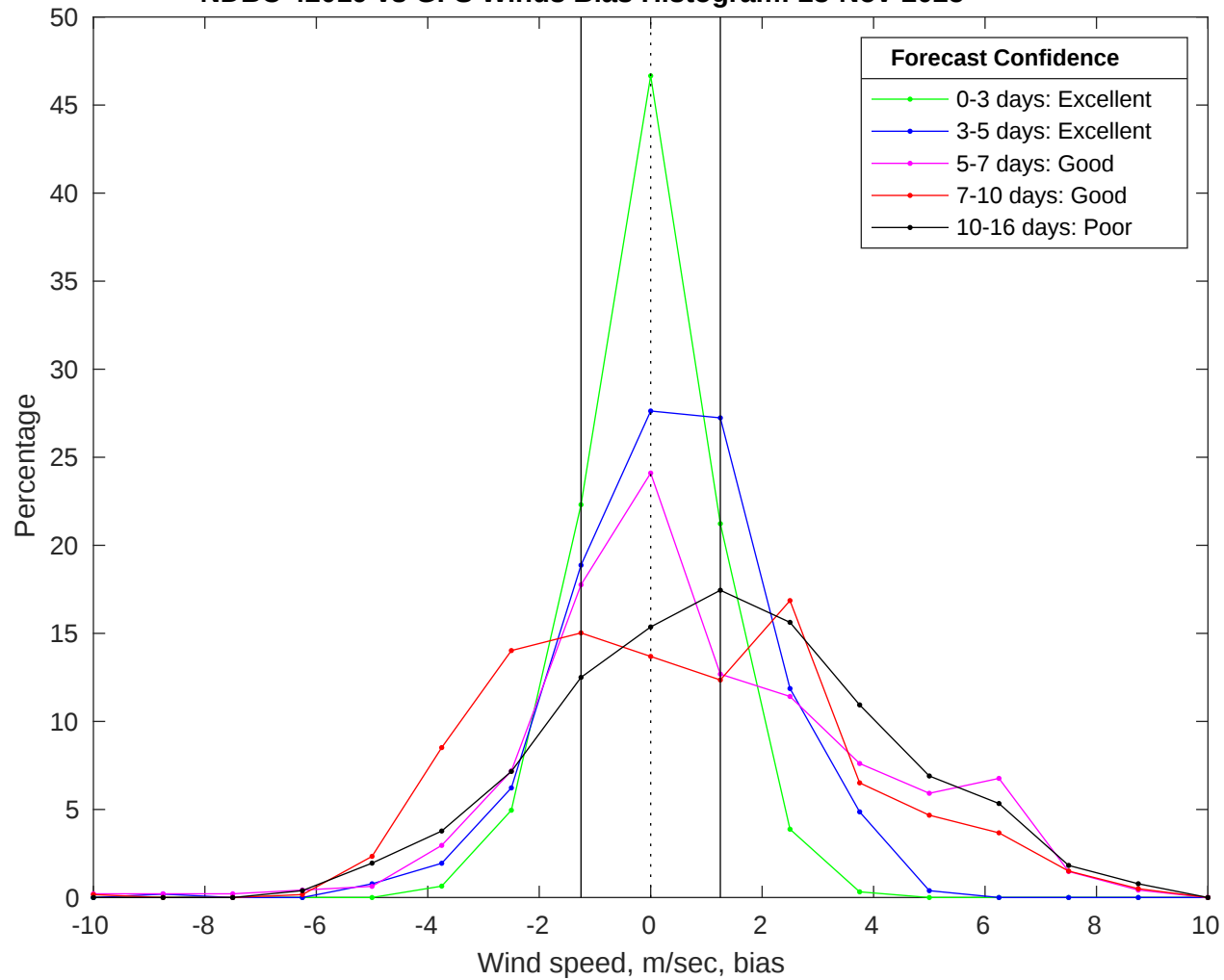
NDBC 42019 vs GFS Winds Bias Histogram: 23-Nov-2025
