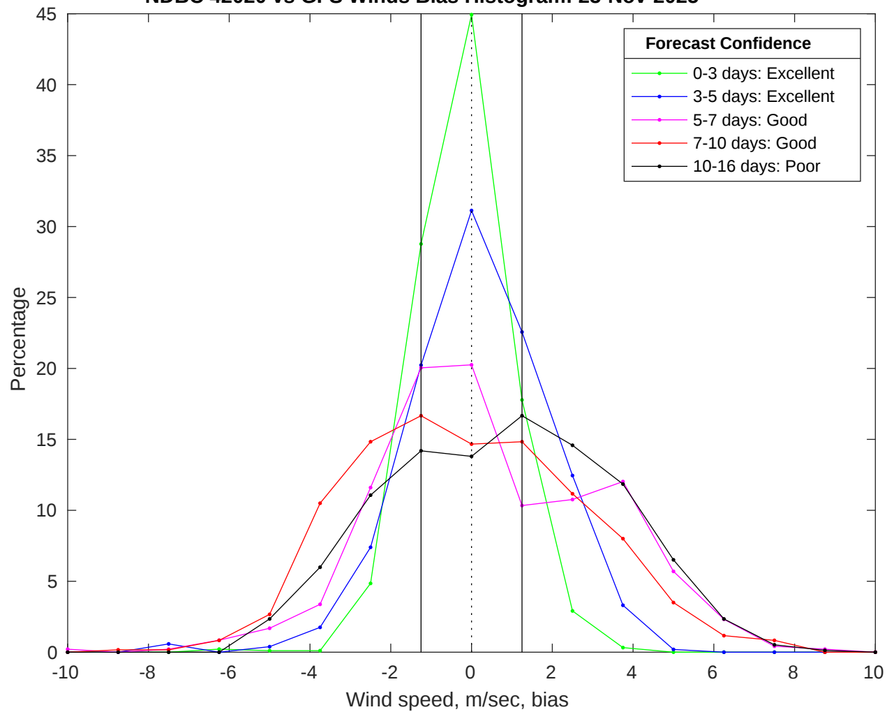
NDBC 42020 vs GFS Winds Bias Histogram: 23-Nov-2025
