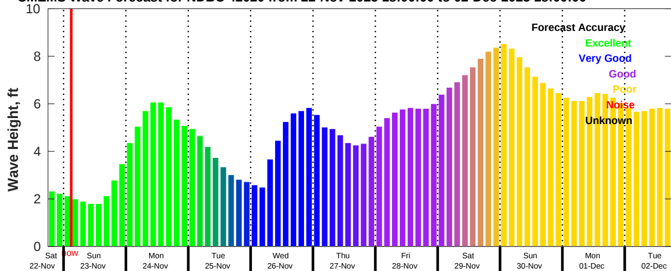
CMEMS Wave Forecast for NDBC 42020 from 22-Nov-2025 18:00:00 to 02-Dec-2025 18:00:00
