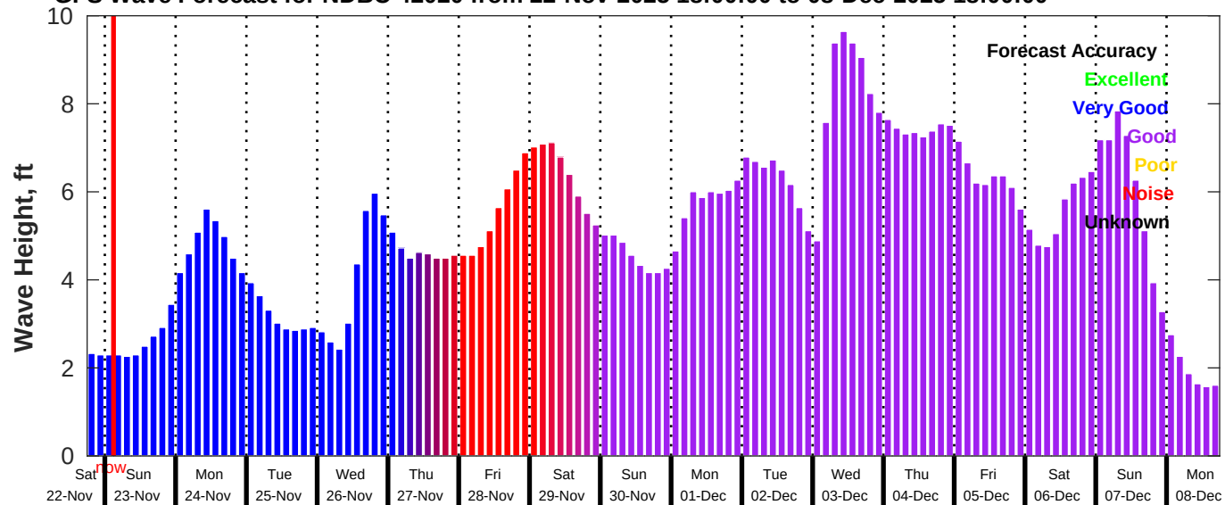
GFS Wave Forecast for NDBC 42020 from 22-Nov-2025 18:00:00 to 08-Dec-2025 18:00:00
