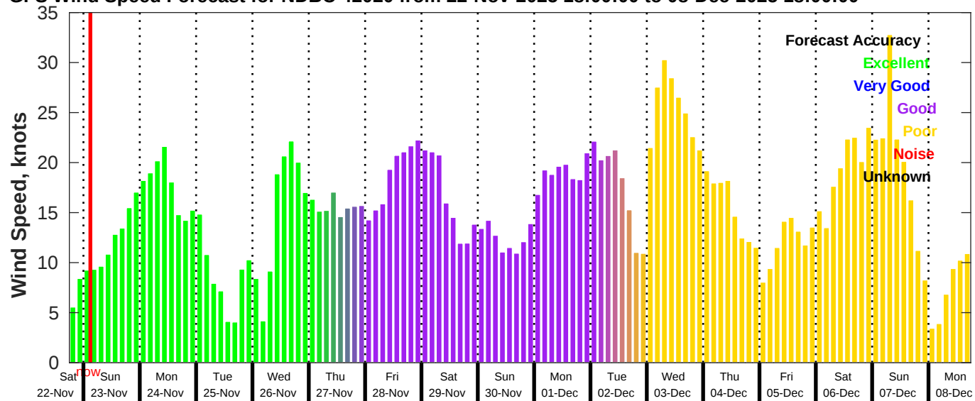
GFS Wind Speed Forecast for NDBC 42020 from 22-Nov-2025 18:00:00 to 08-Dec-2025 18:00:00
