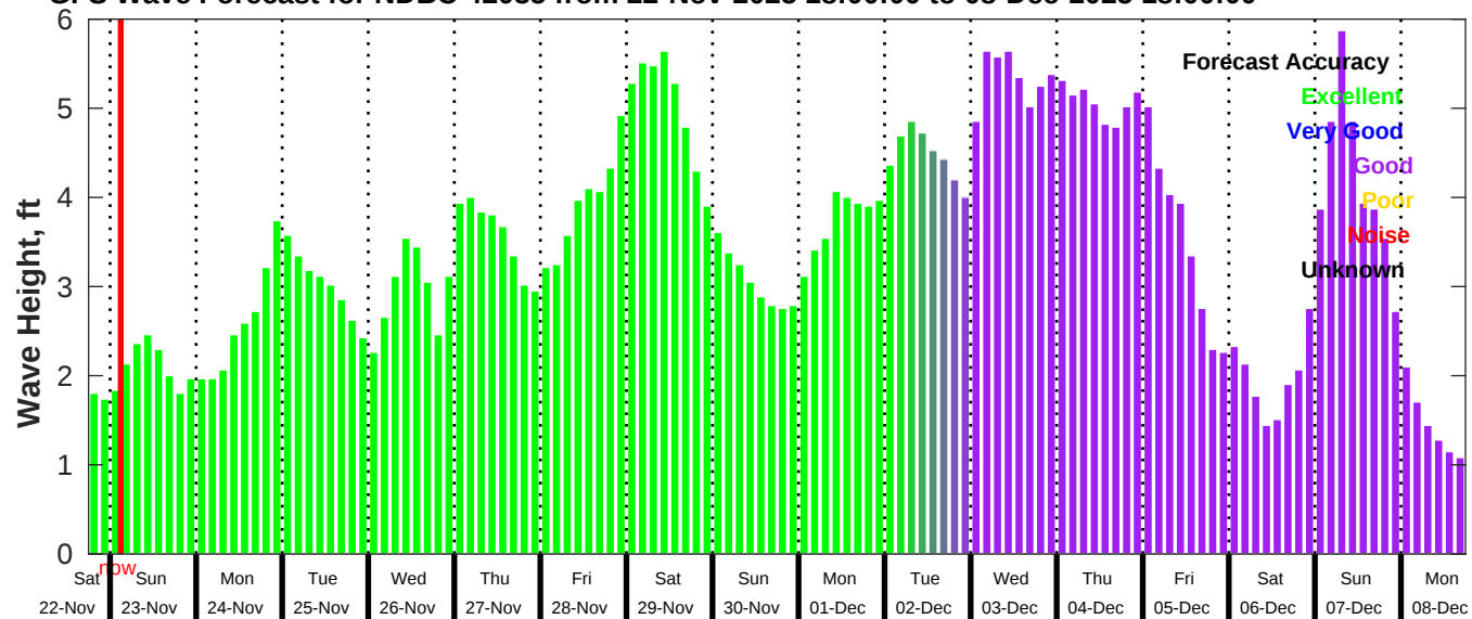
GFS Wave Forecast for NDBC 42035 from 22-Nov-2025 18:00:00 to 08-Dec-2025 18:00:00
