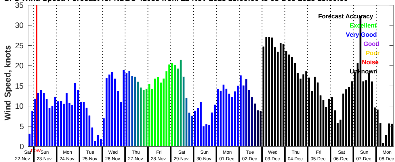
GFS Wind Speed Forecast for NDBC 42035 from 22-Nov-2025 18:00:00 to 08-Dec-2025 18:00:00
