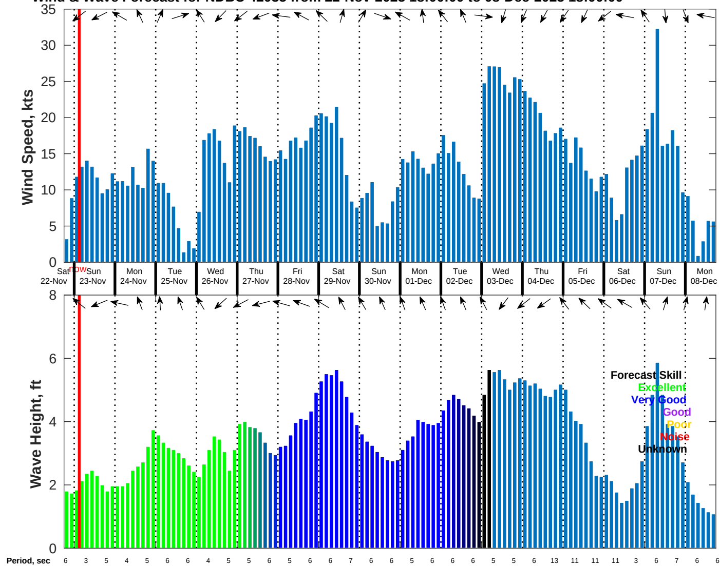
Wind & Wave Forecast for NDBC 42035 from 22-Nov-2025 18:00:00 to 08-Dec-2025 18:00:00
