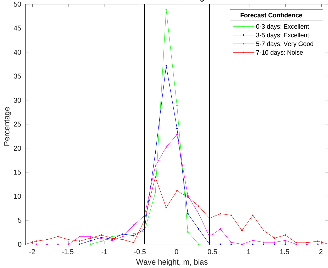
NDBC 42036 vs CMEMS Waves Bias Histogram: 23-Nov-2025
