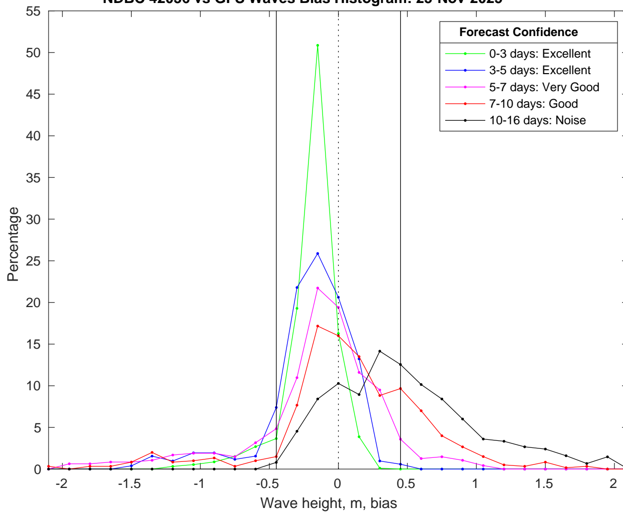
NDBC 42036 vs GFS Waves Bias Histogram: 23-Nov-2025
