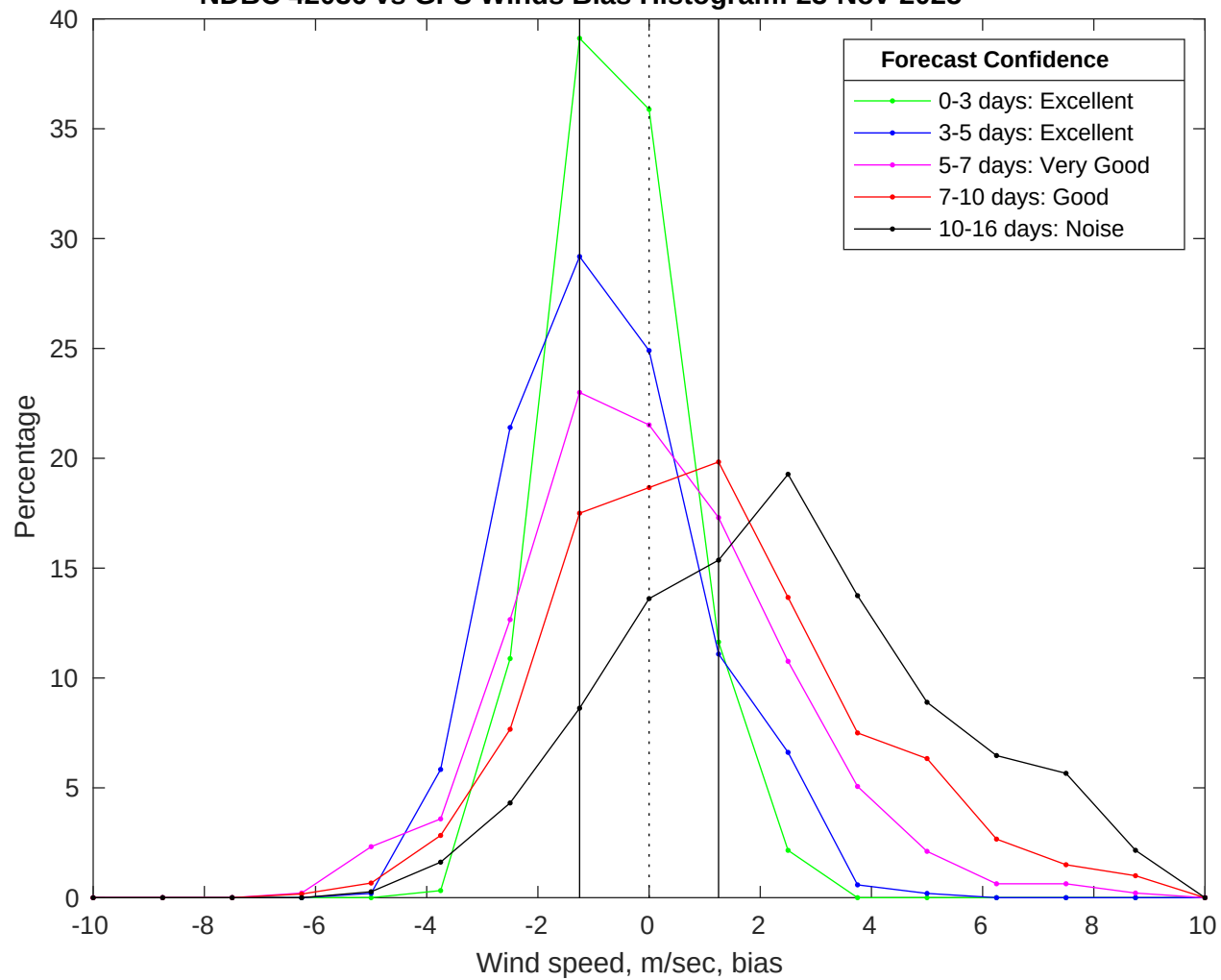
NDBC 42036 vs GFS Winds Bias Histogram: 23-Nov-2025
