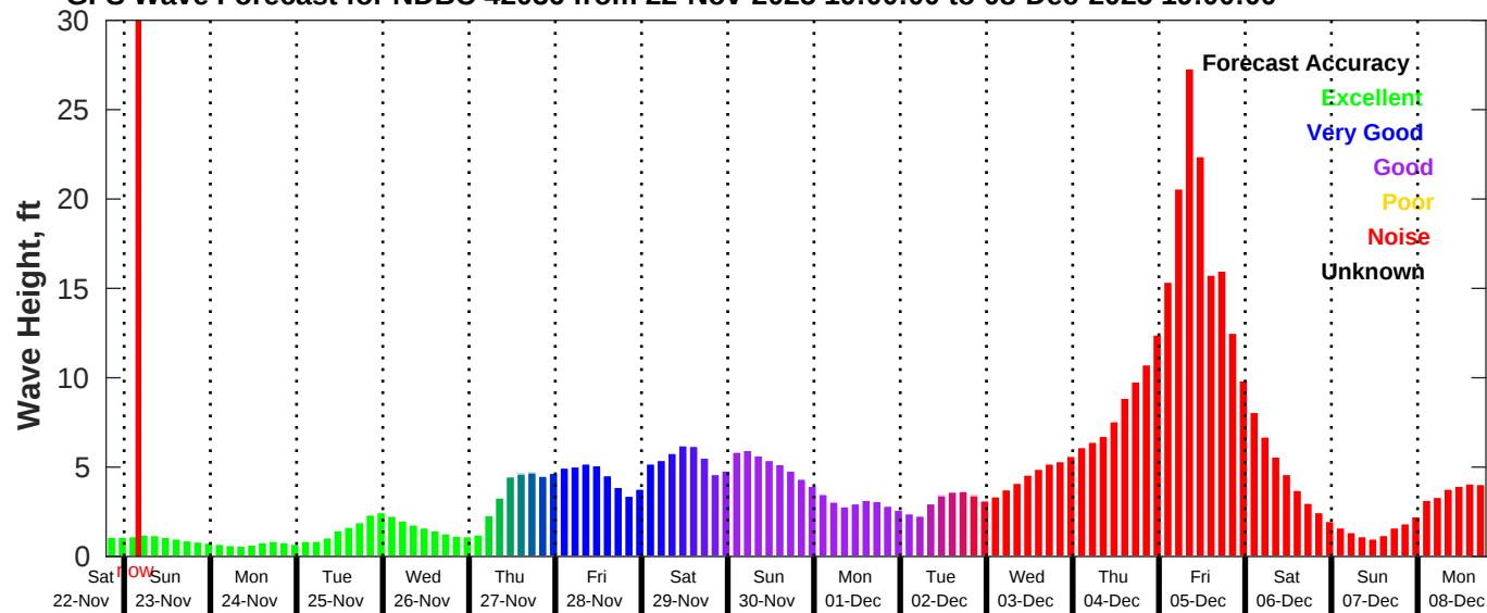
GFS Wave Forecast for NDBC 42036 from 22-Nov-2025 19:00:00 to 08-Dec-2025 19:00:00
