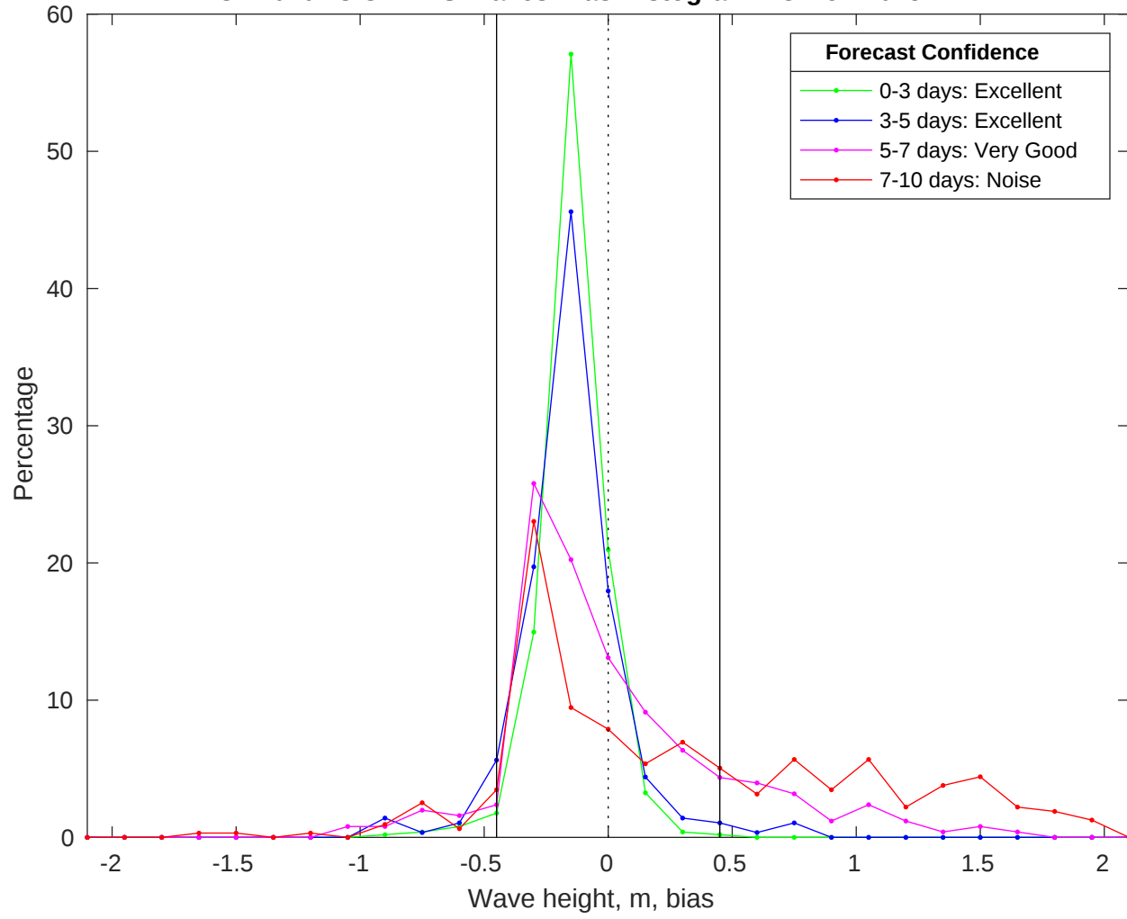
NDBC 42040 vs CMEMS Waves Bias Histogram: 23-Nov-2025
