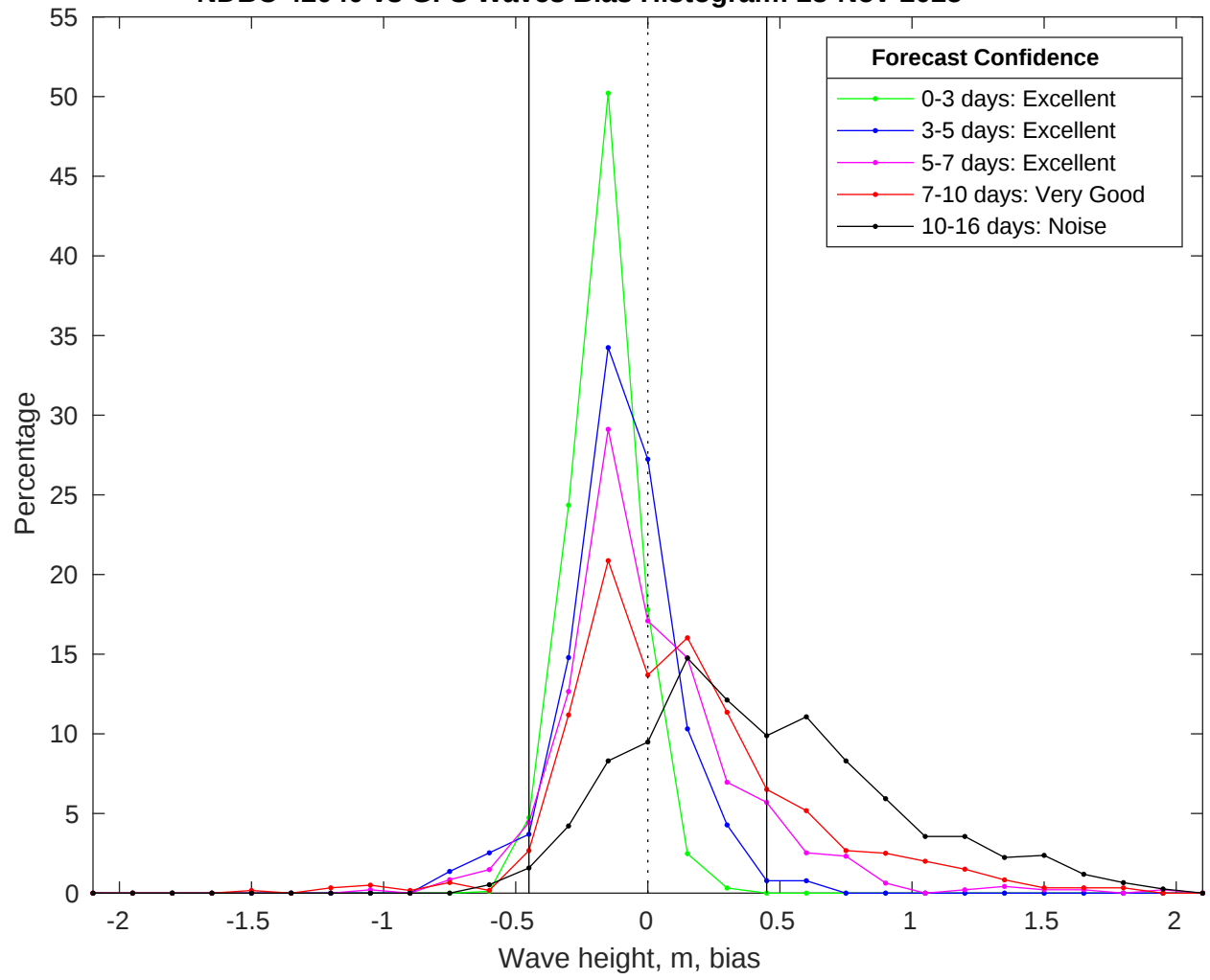
NDBC 42040 vs GFS Waves Bias Histogram: 23-Nov-2025
