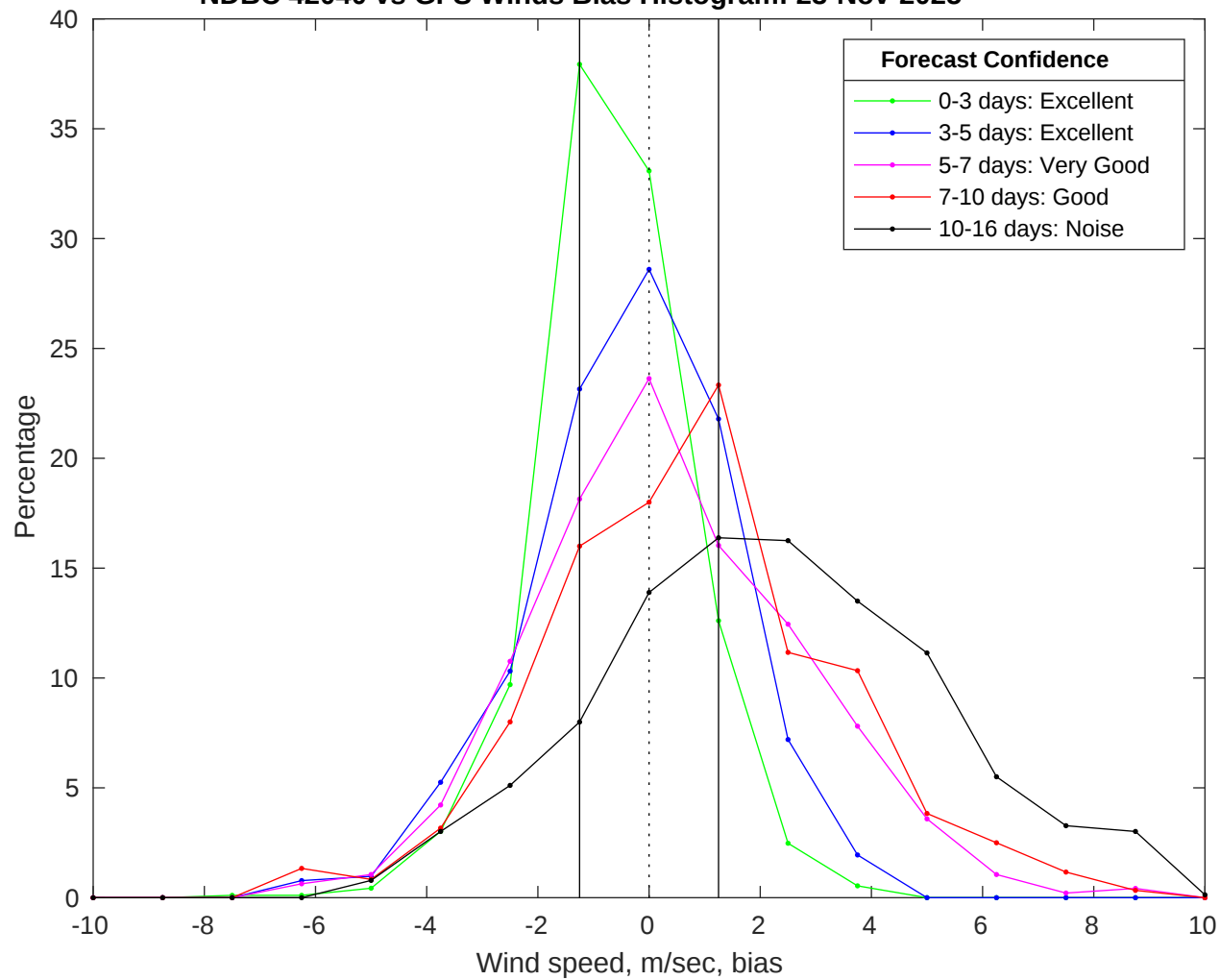
NDBC 42040 vs GFS Winds Bias Histogram: 23-Nov-2025
