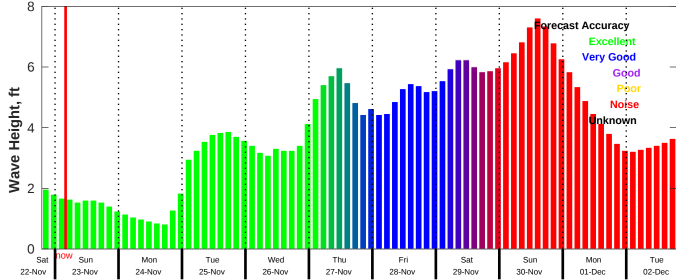
CMEMS Wave Forecast for NDBC 42040 from 22-Nov-2025 19:00:00 to 02-Dec-2025 19:00:00
