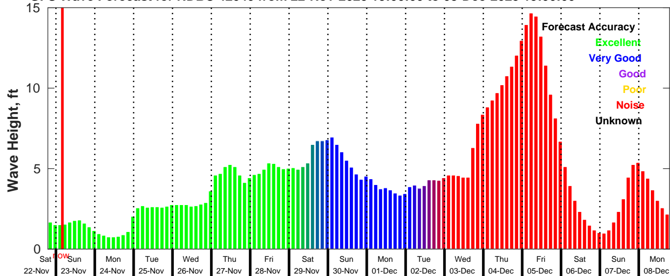
GFS Wave Forecast for NDBC 42040 from 22-Nov-2025 19:00:00 to 08-Dec-2025 19:00:00
