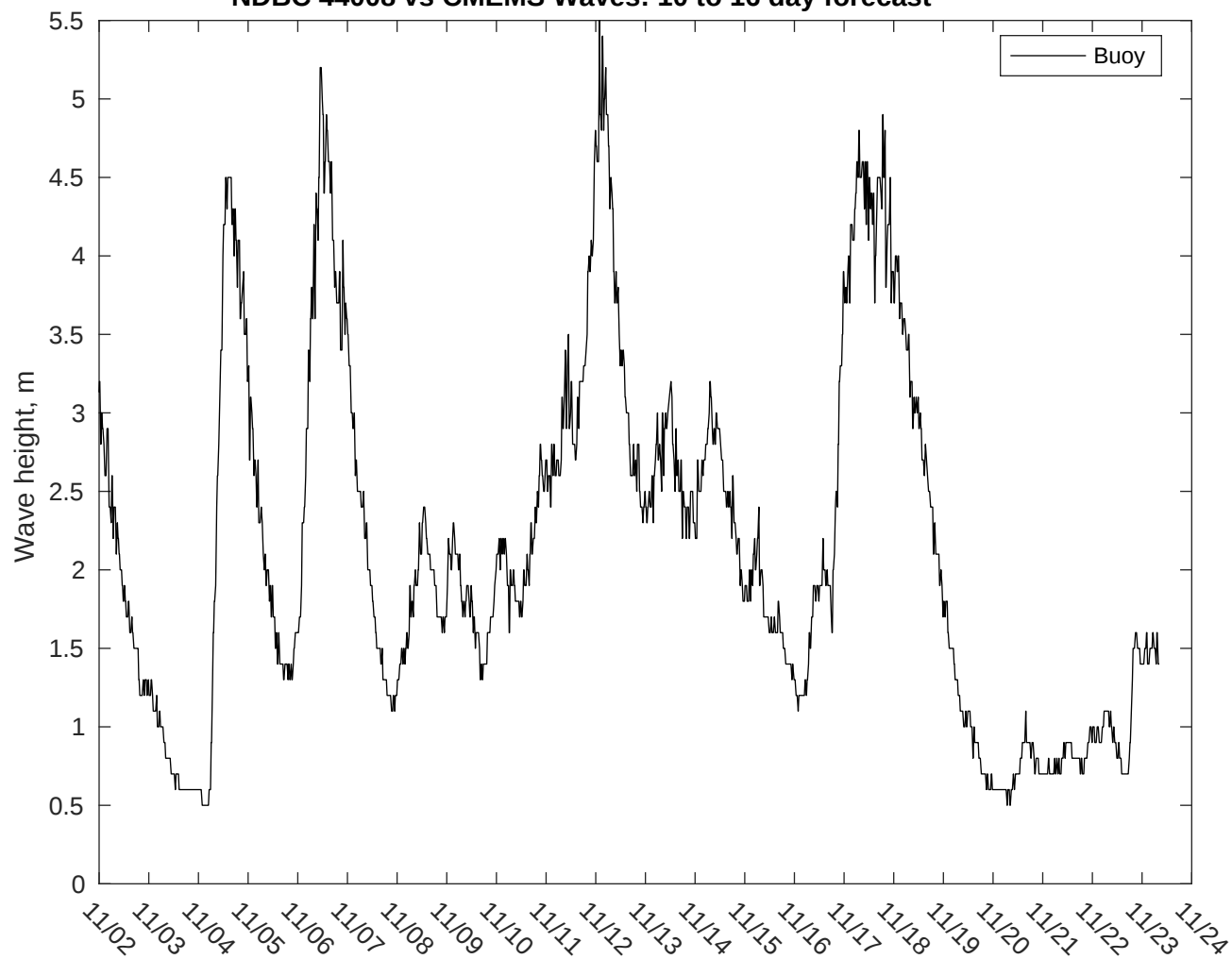
NDBC 44008 vs CMEMS Waves: 10 to 16 day forecast
