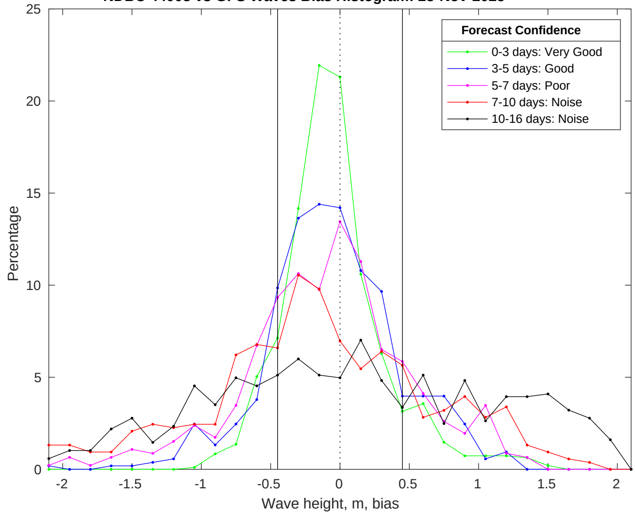
NDBC 44008 vs GFS Waves Bias Histogram: 23-Nov-2025
