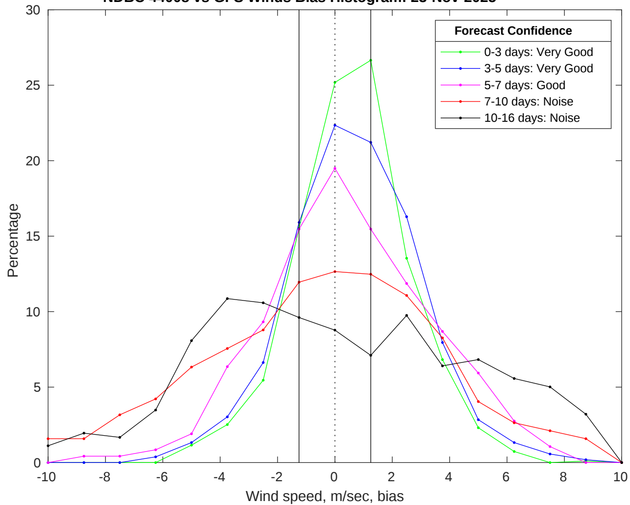
NDBC 44008 vs GFS Winds Bias Histogram: 23-Nov-2025
